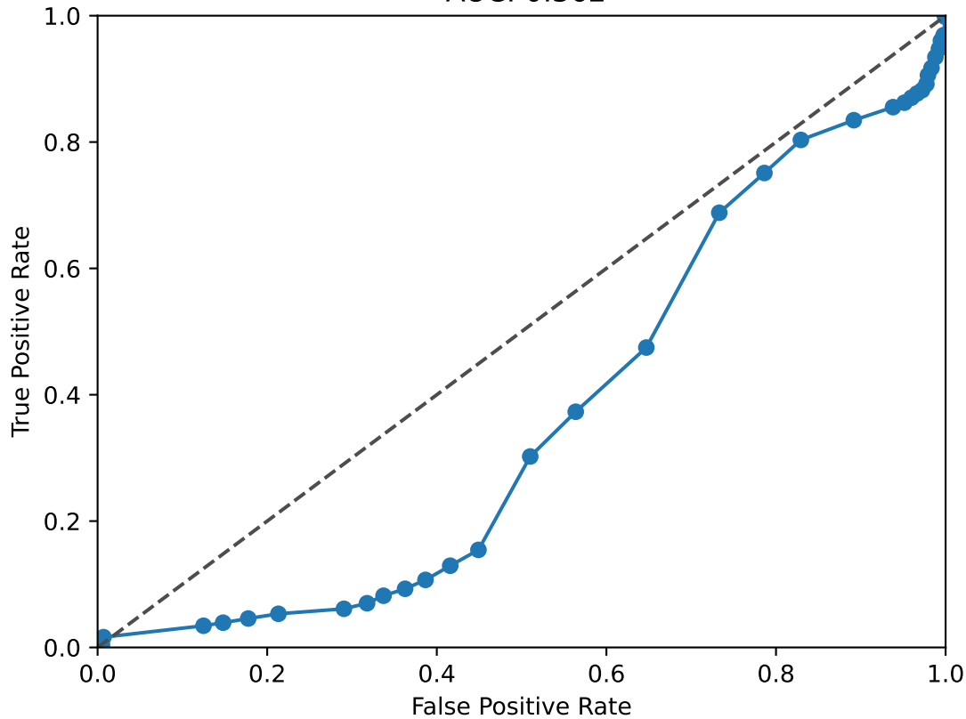
PBX1 ROC Curve AUC: 0.362
