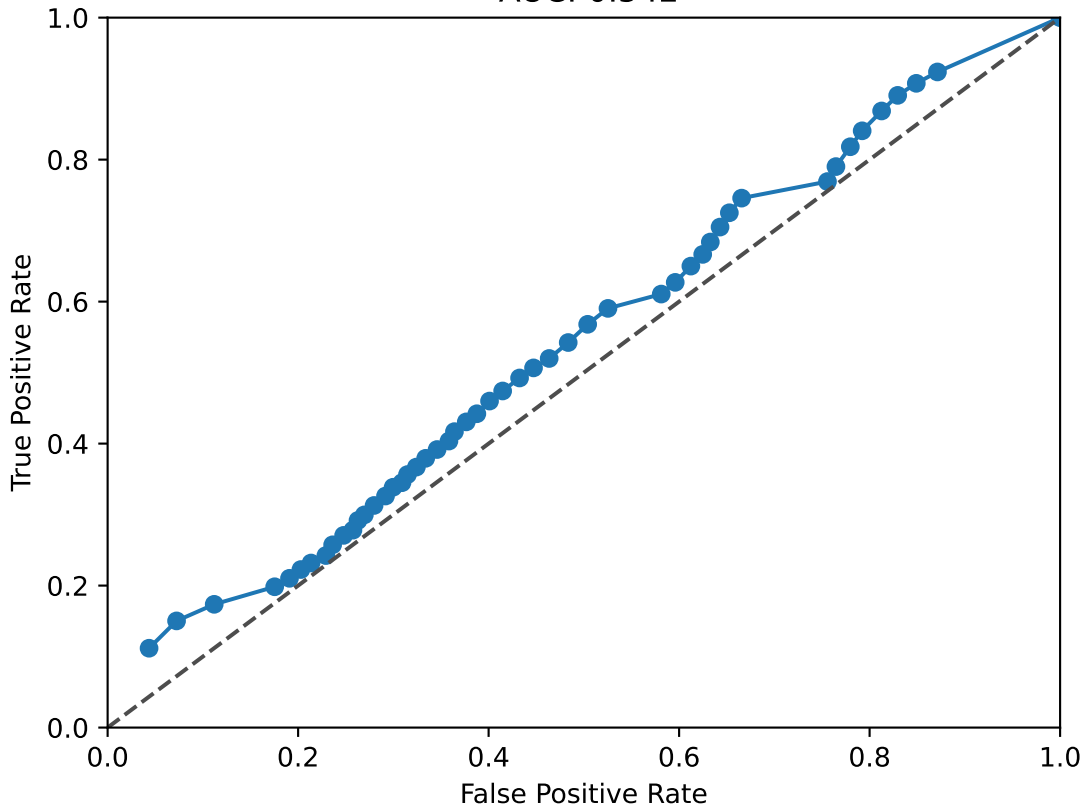
RORA_RORB ROC Curve AUC: 0.542
