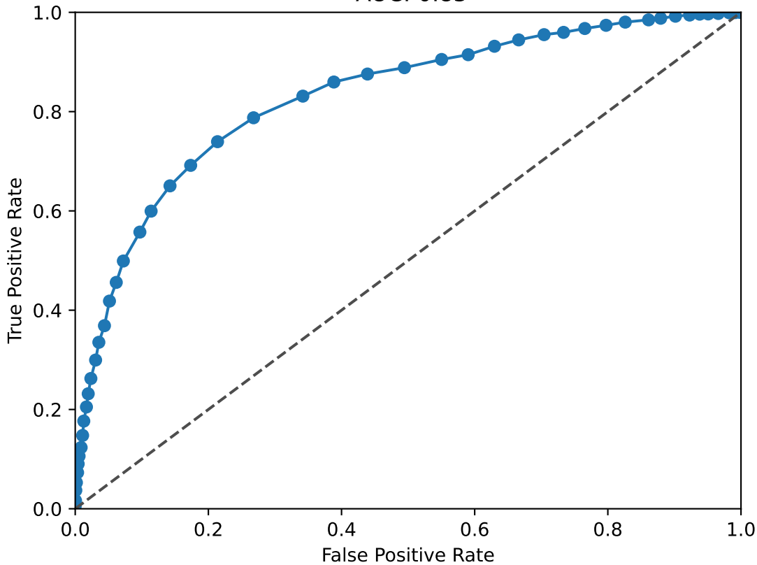
SIX4 ROC Curve AUC: 0.83
