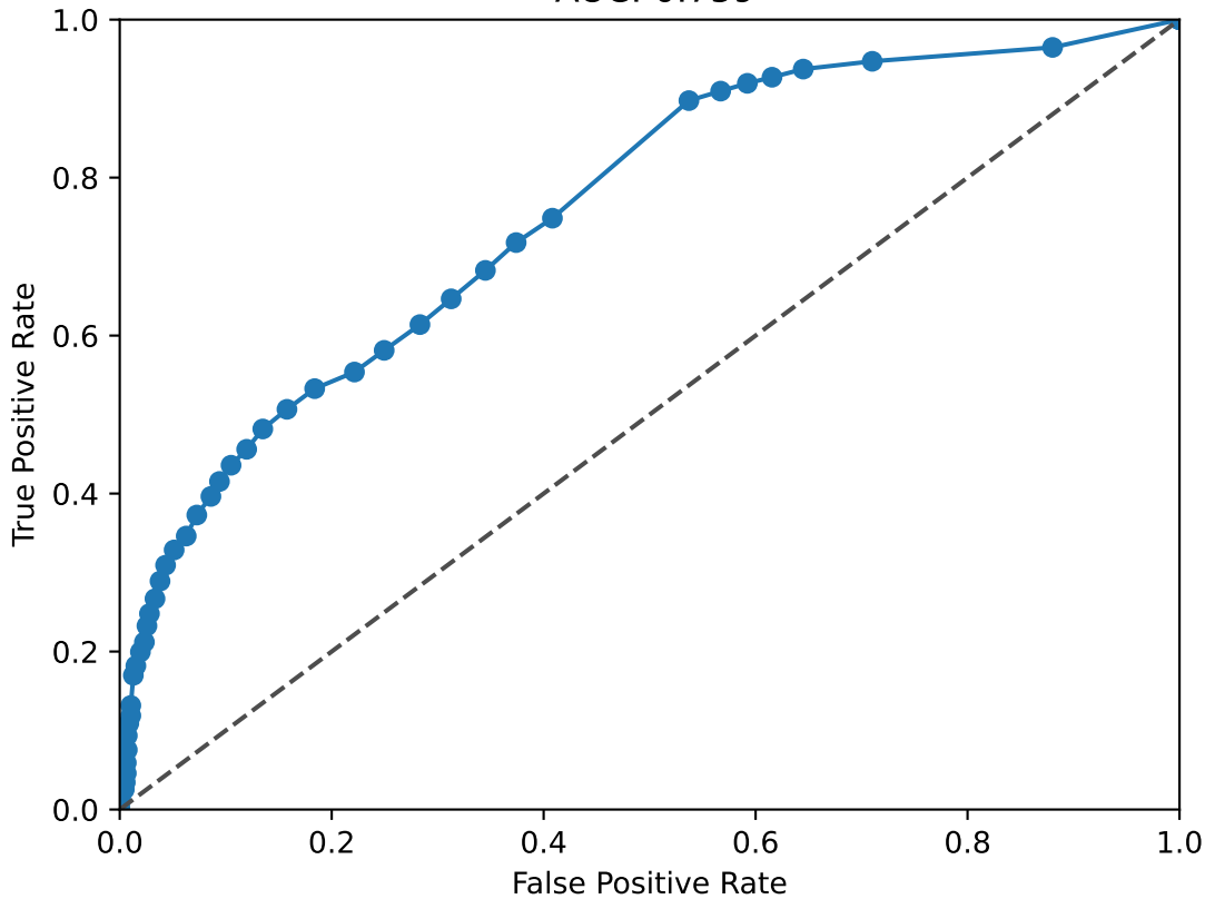
SOX11 ROC Curve AUC: 0.759
