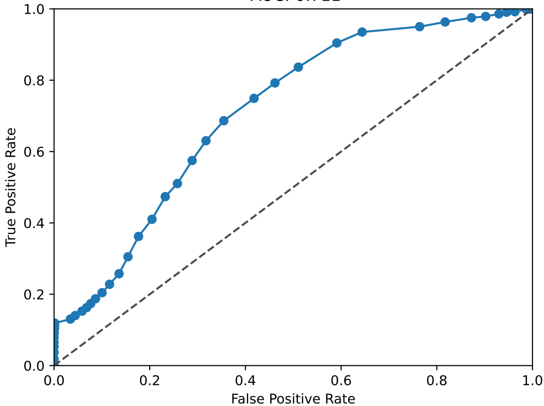
STAT2 ROC Curve AUC: 0.711
