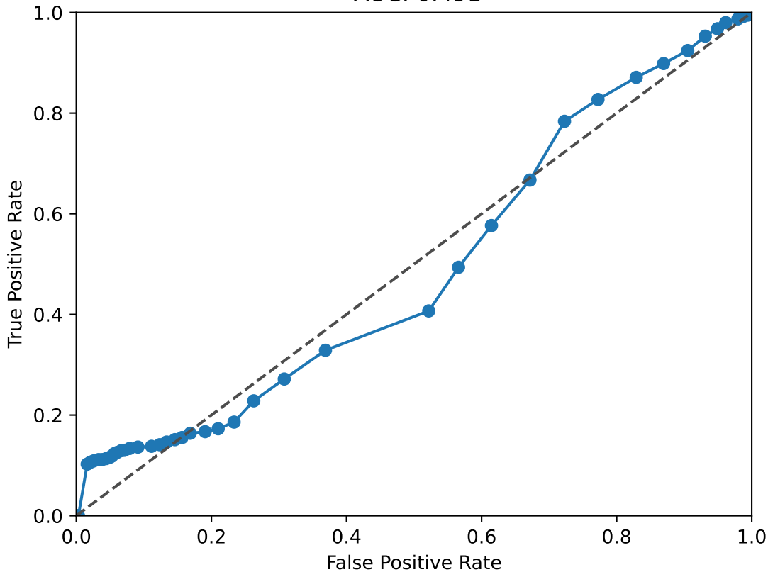
TCF7L1 ROC Curve AUC: 0.491
