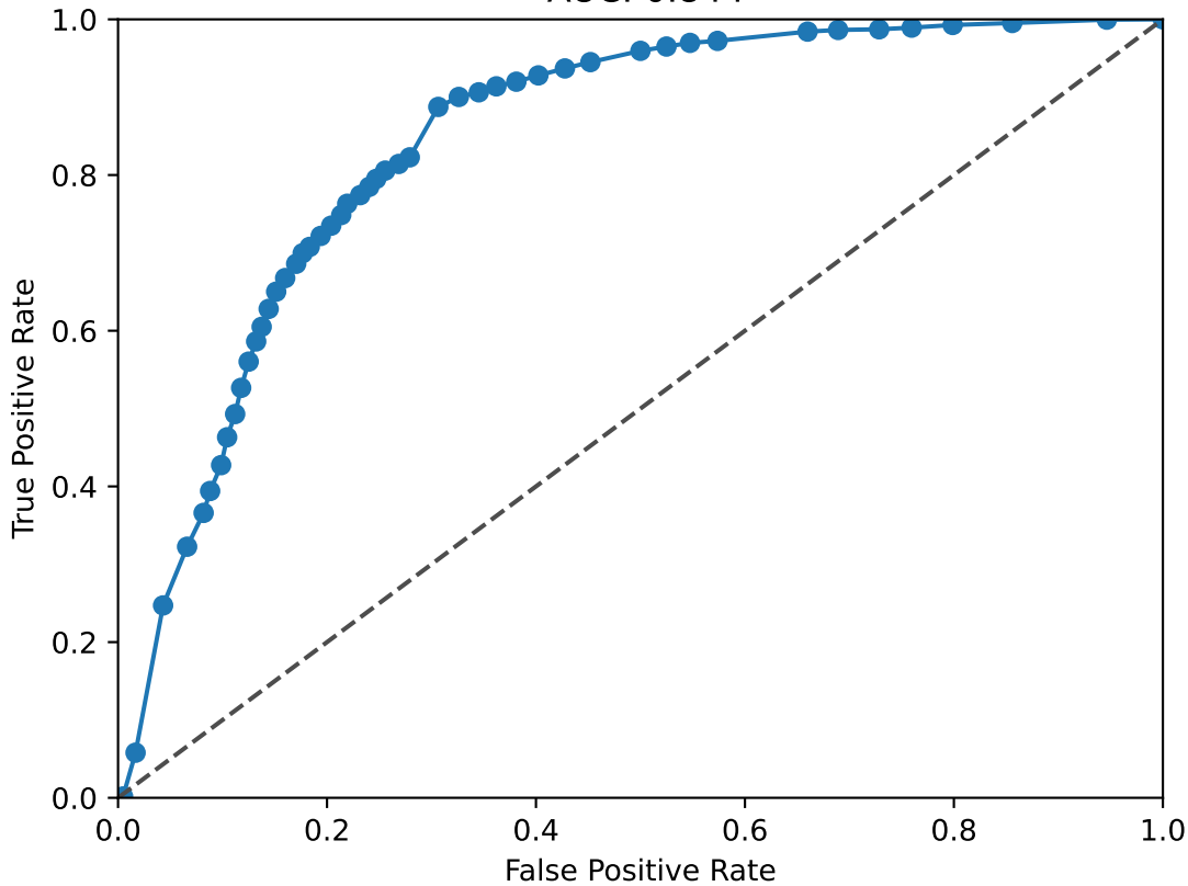
TEAD1 ROC Curve AUC: 0.844
