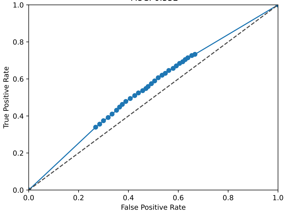
THR B ROC Curve AUC: 0.552
