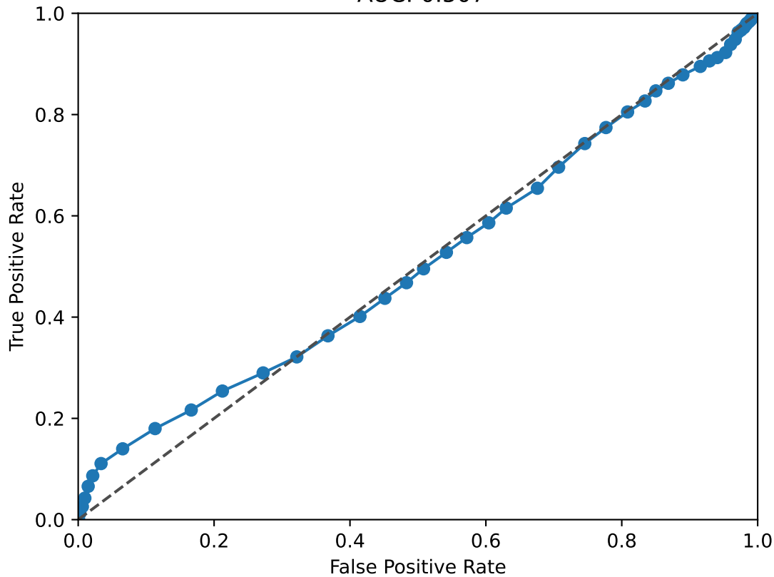
EGR1 ROC Curve AUC: 0.507
