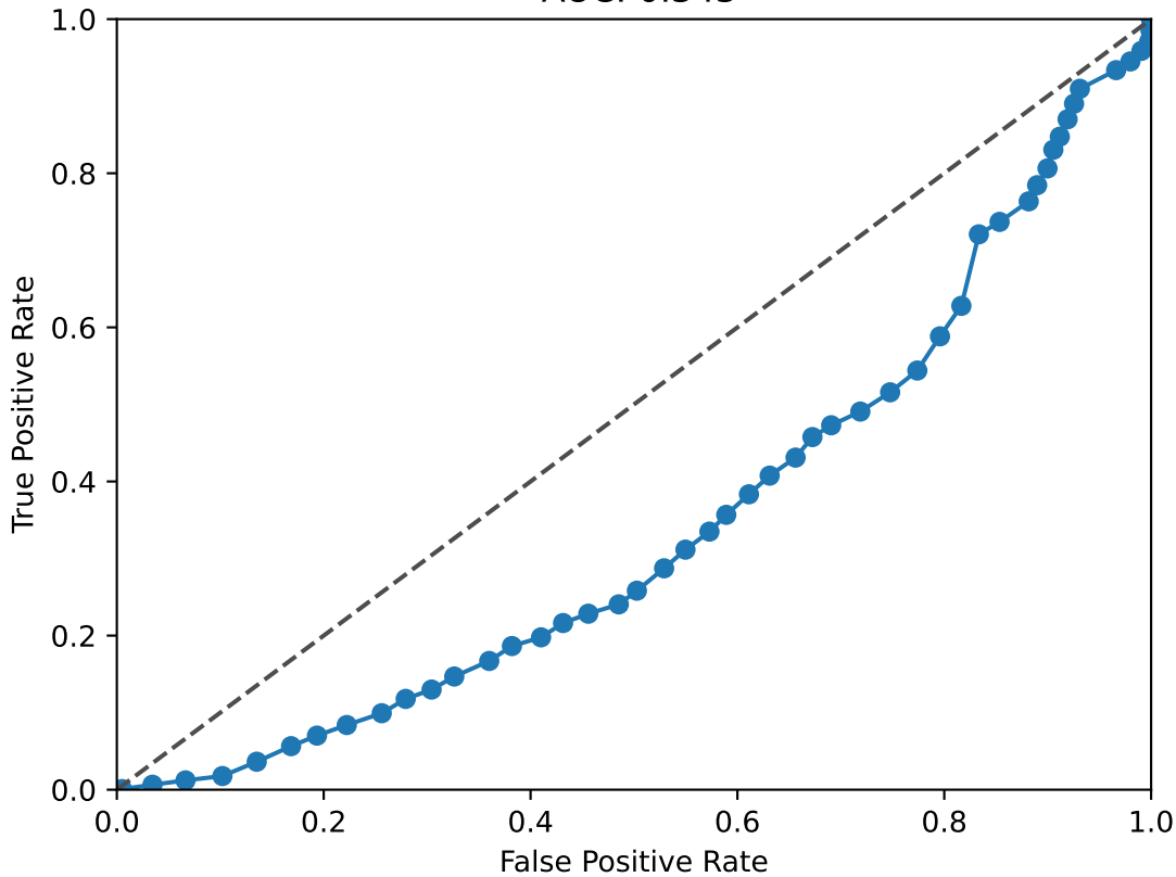
EPCAM ROC Curve AUC: 0.343
