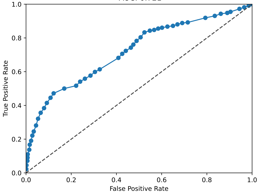
ETS1 ROC Curve AUC: 0.721
