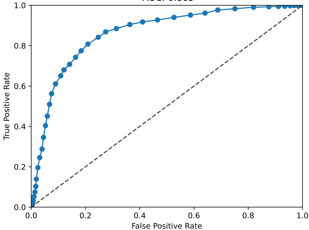
FOS ROC Curve AUC: 0.863
