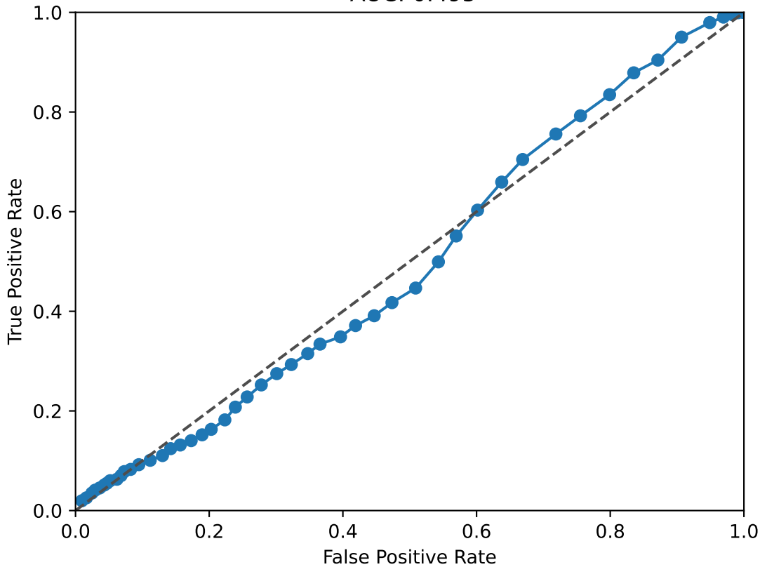
ICAM1 ROC Curve AUC: 0.495
