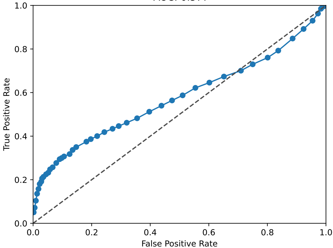
RUNX1 ROC Curve AUC: 0.577
