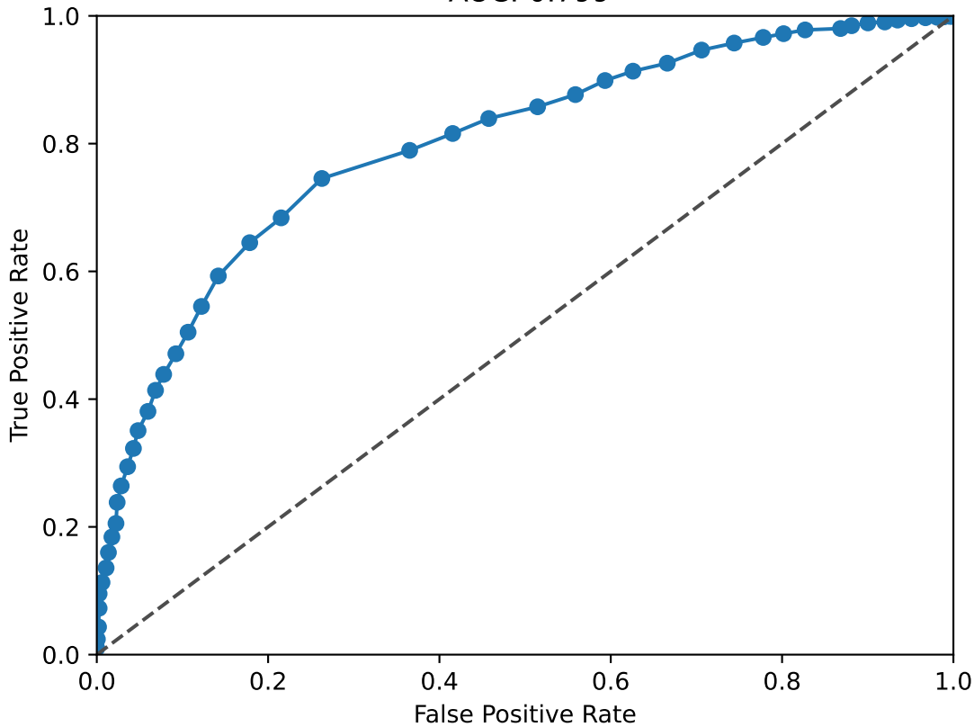
SIX4 ROC Curve AUC: 0.799
