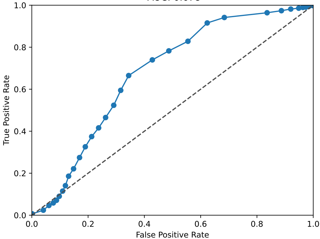
STAT2 ROC Curve AUC: 0.678
