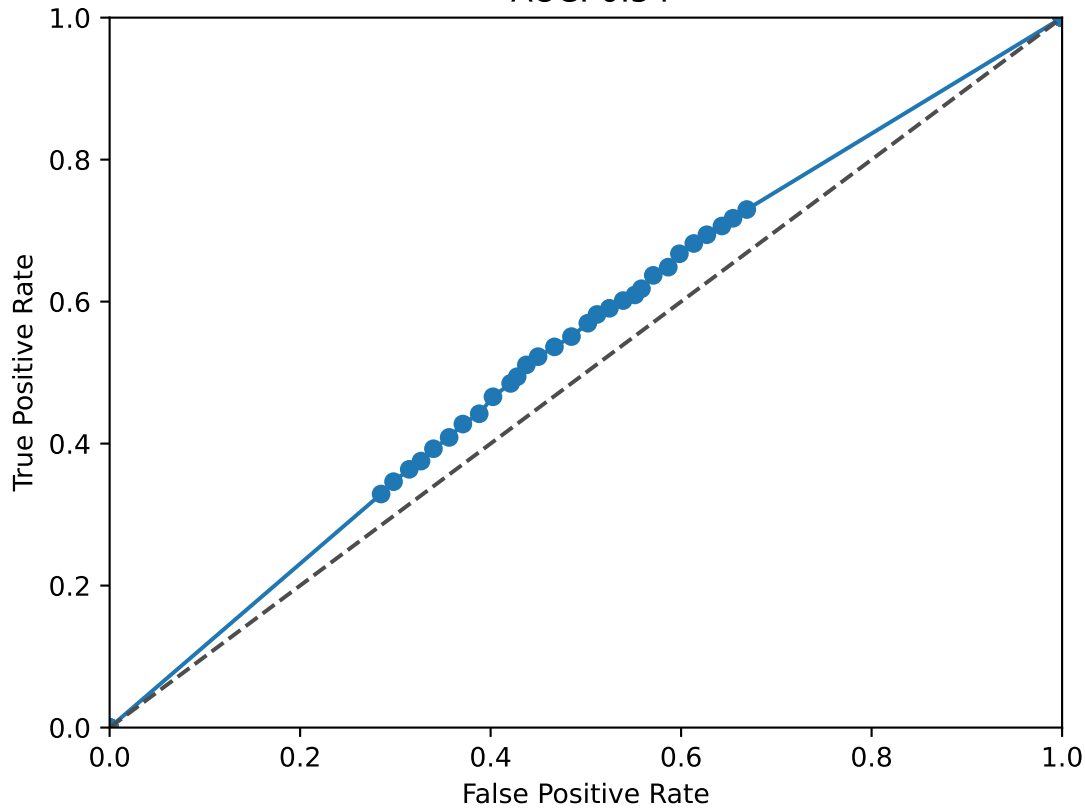
THR B ROC Curve AUC: 0.54
