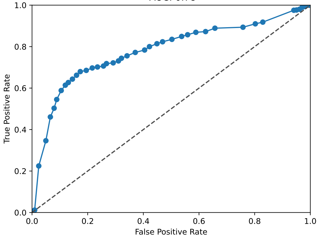
BACH1 ROC Curve AUC: 0.78
