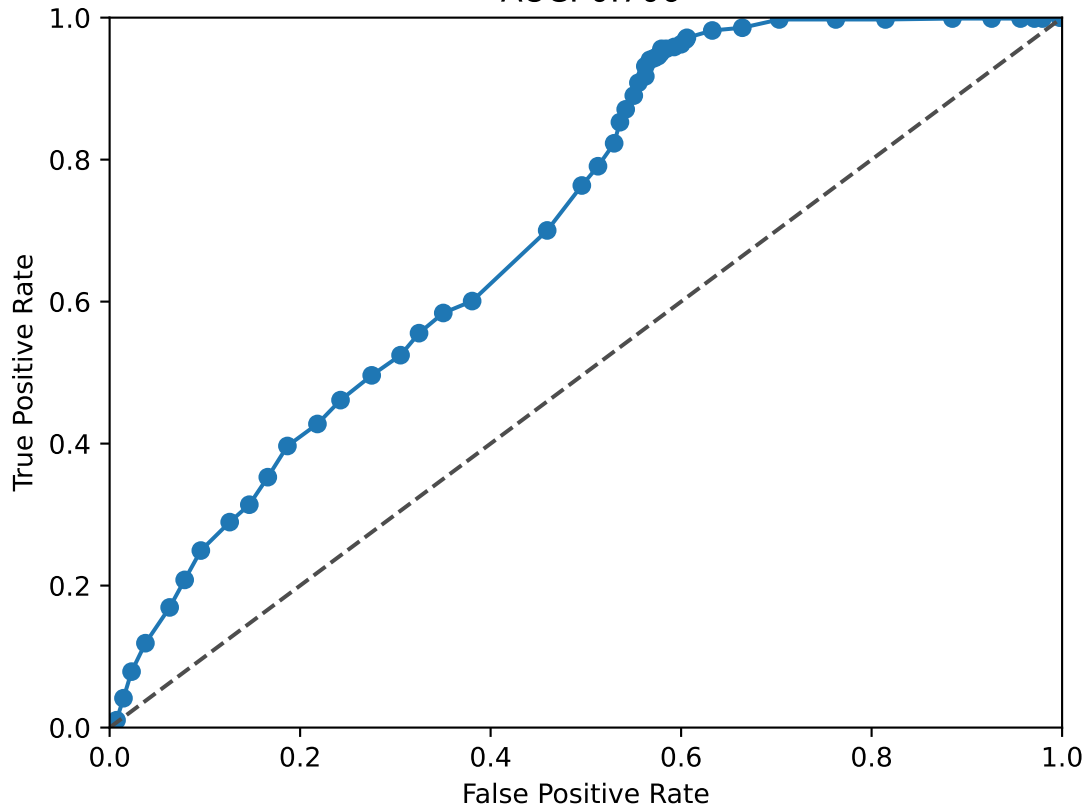
CUX2 ROC Curve AUC: 0.706
