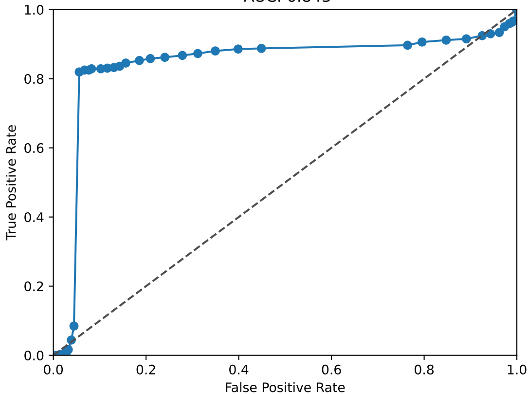
EHF ROC Curve AUC: 0.843
