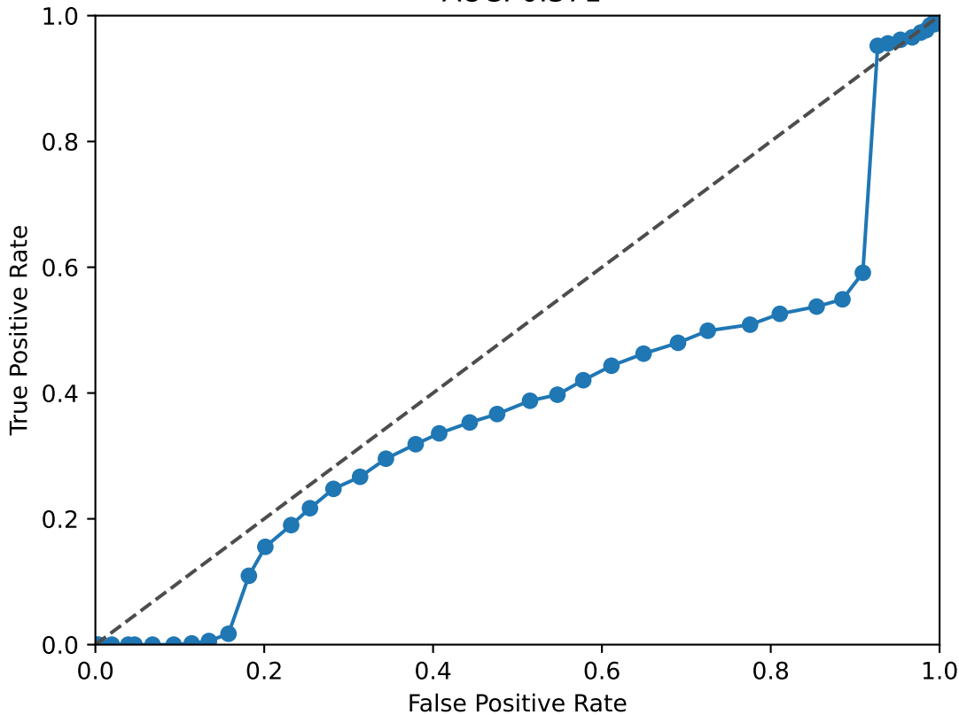
EPCAM ROC Curve AUC: 0.371
