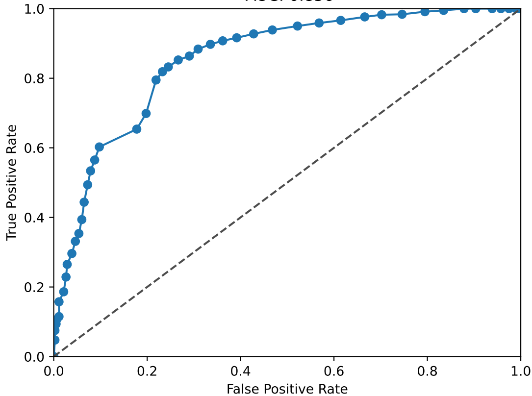
FOS ROC Curve AUC: 0.856
