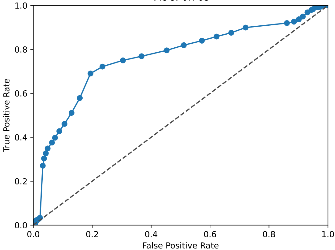
HES1 ROC Curve AUC: 0.763
