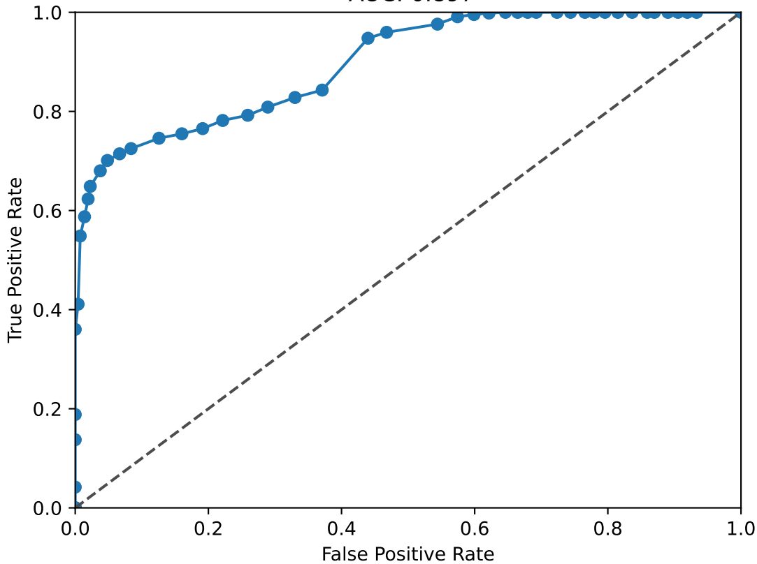
JUNB ROC Curve AUC: 0.897
