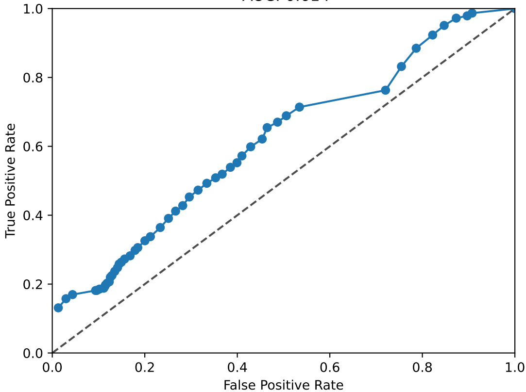
RORA_RORB ROC Curve AUC: 0.614
