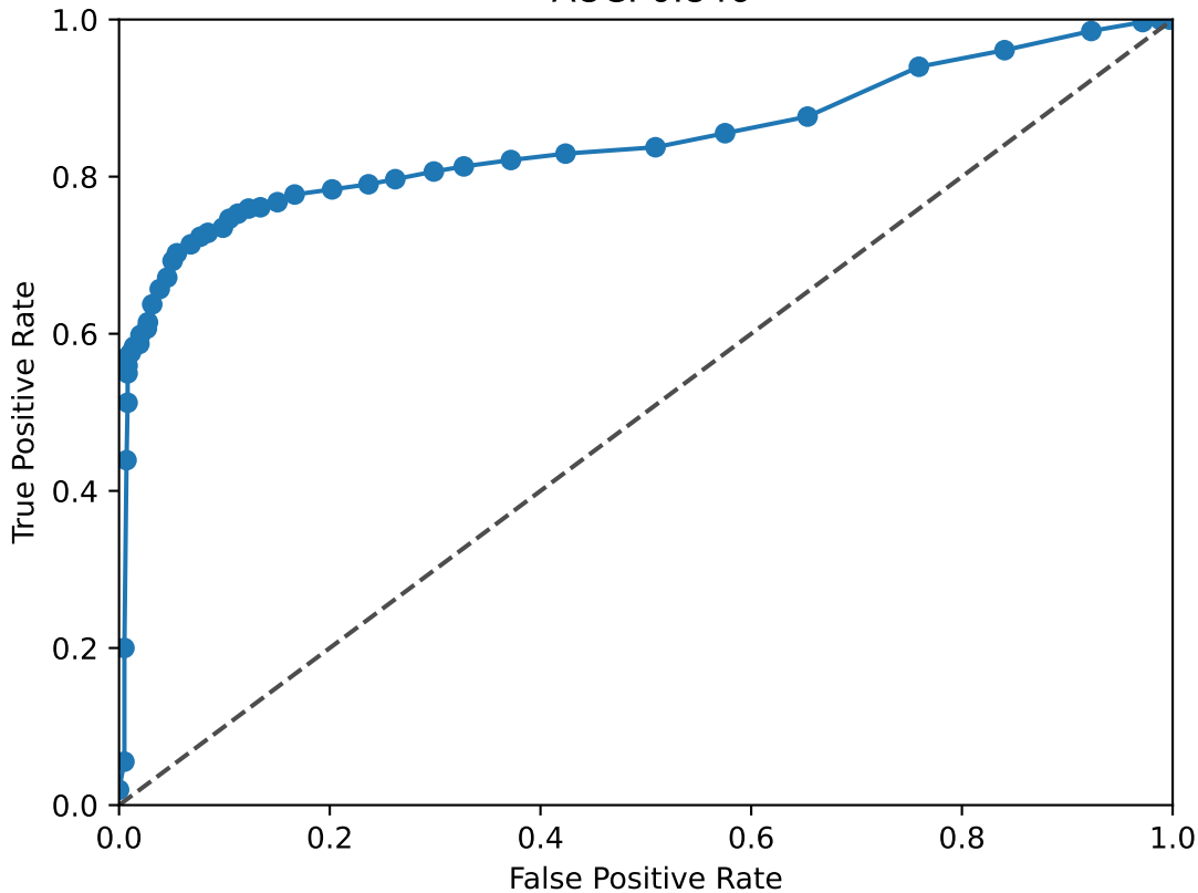
RUNX1 ROC Curve AUC: 0.846
