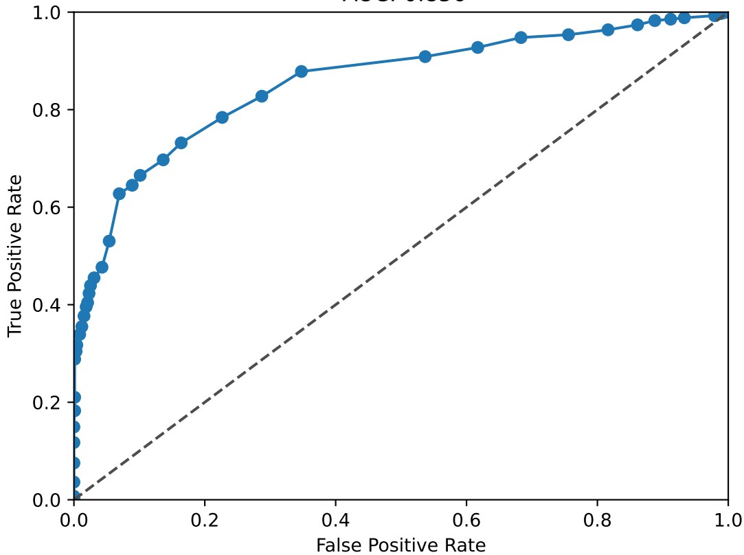
STAT2 ROC Curve AUC: 0.856
