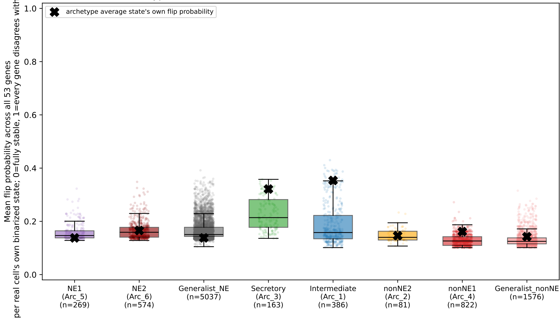
Per-cell flip probability by GEMM phenotype label (archetype AVERAGE states' own values shown as X markers, for reference)
