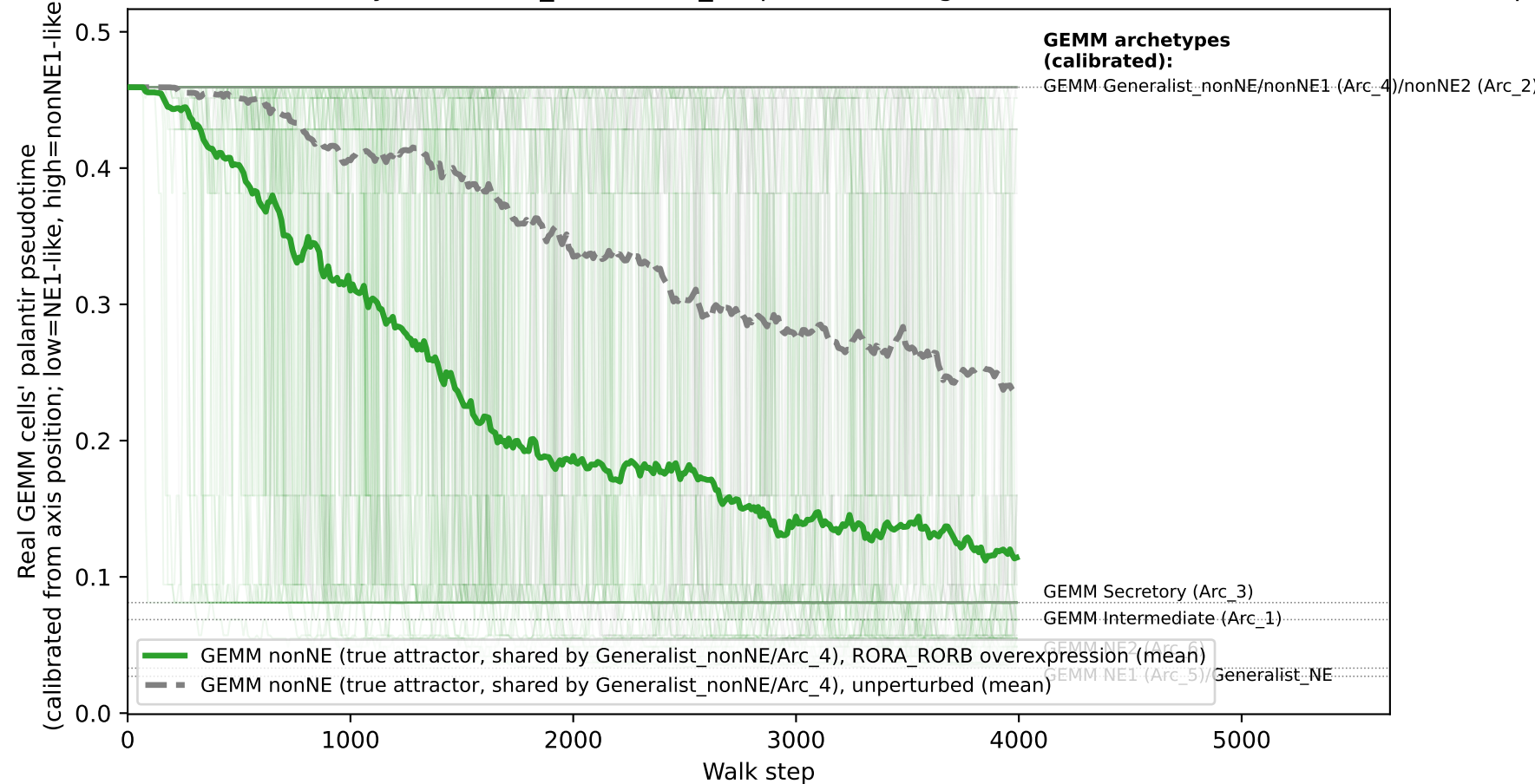
GEMM nonNE (true attractor, shared by Generalist_nonNE/Arc_4): position along NE1<->nonNE1 axis, calibrated to real pseudotime
