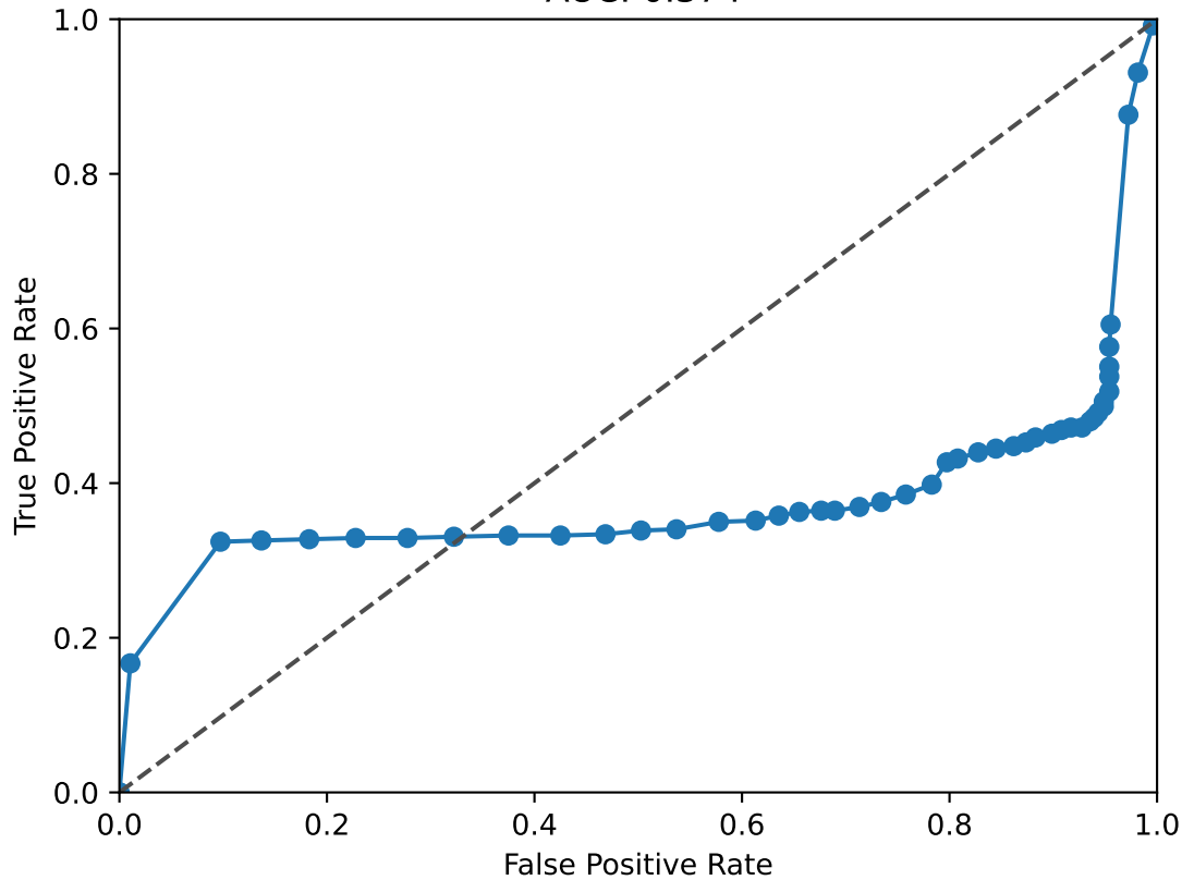
BACH1 ROC Curve AUC: 0.374
