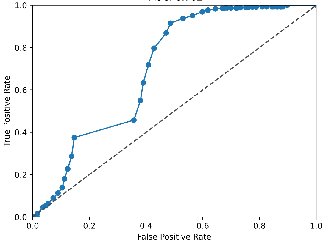
FOXO3 ROC Curve AUC: 0.702
