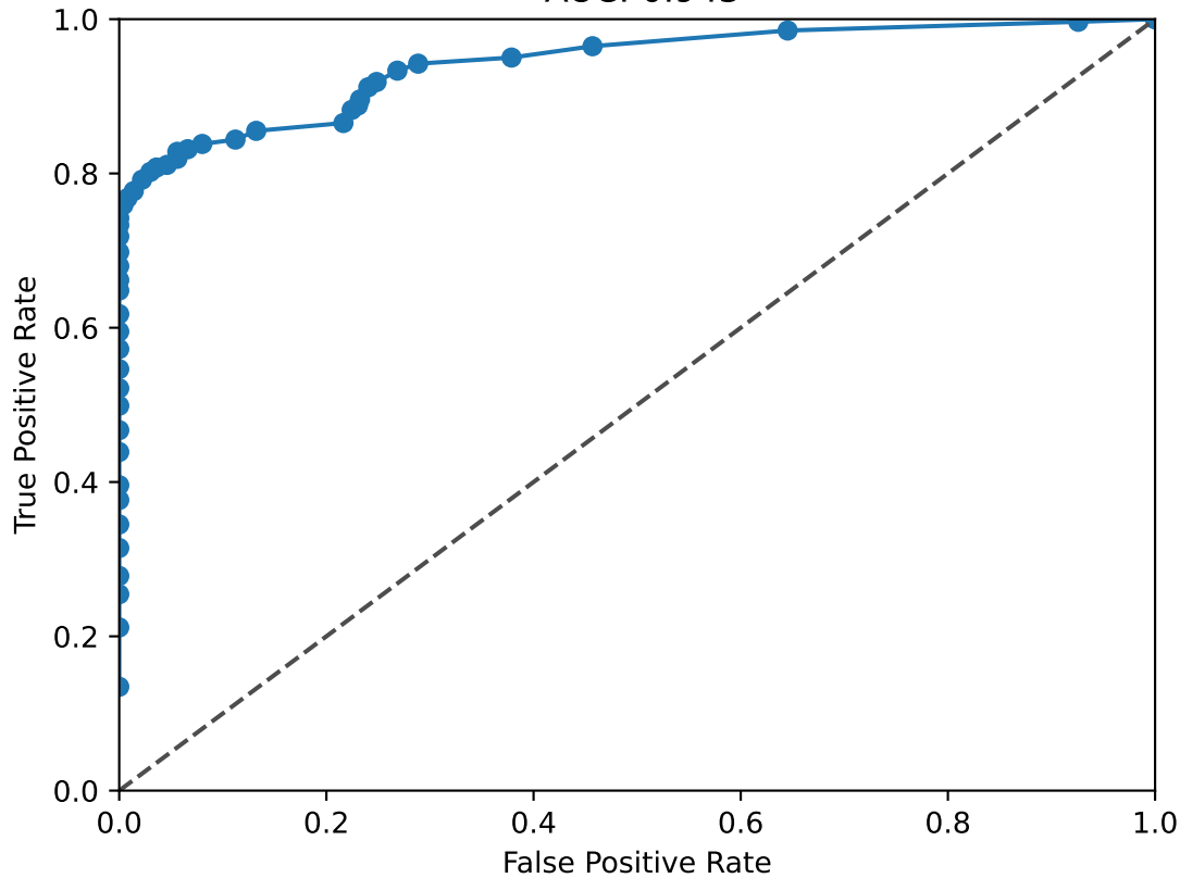
HSF2 ROC Curve AUC: 0.943
