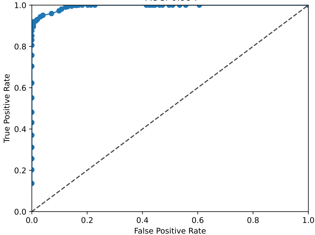
LMX1B ROC Curve AUC: 0.994
