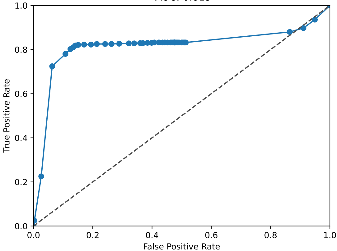
NFATC2 ROC Curve AUC: 0.815
