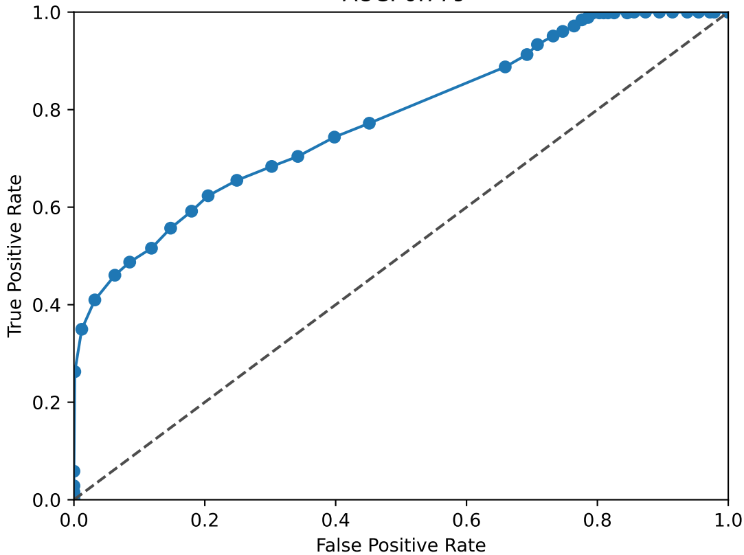
NFIA ROC Curve AUC: 0.779
