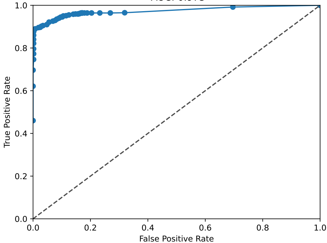
RORA_RORB ROC Curve AUC: 0.973
