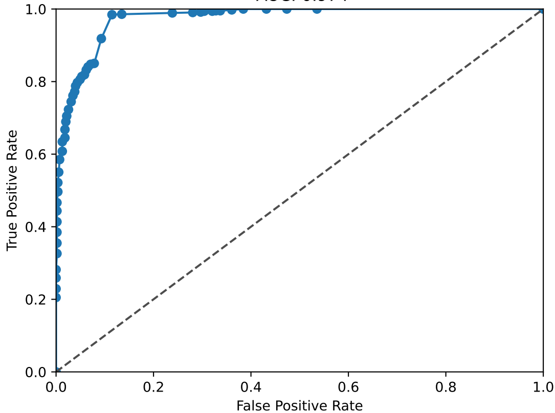
SIX1 ROC Curve AUC: 0.974
