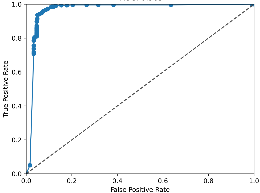
SMAD3 ROC Curve AUC: 0.965
