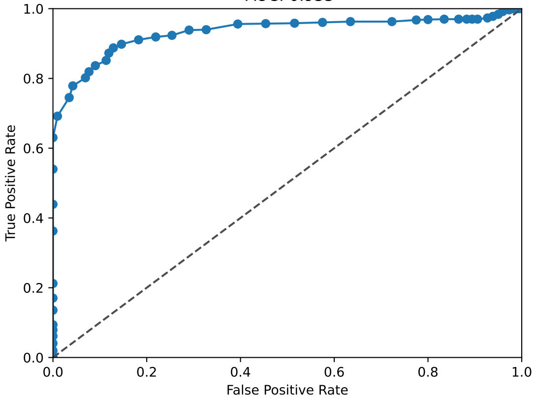
TBX15 ROC Curve AUC: 0.933
