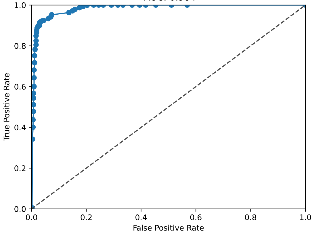
TEAD1 ROC Curve AUC: 0.984
