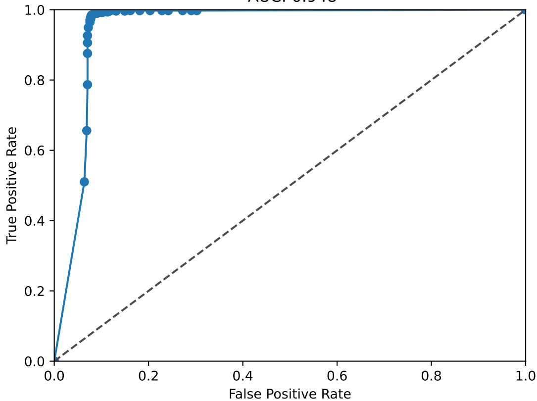
THR B ROC Curve AUC: 0.948
