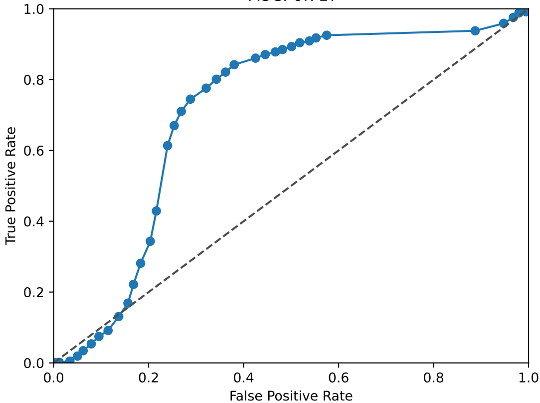
ETS1 ROC Curve AUC: 0.717
