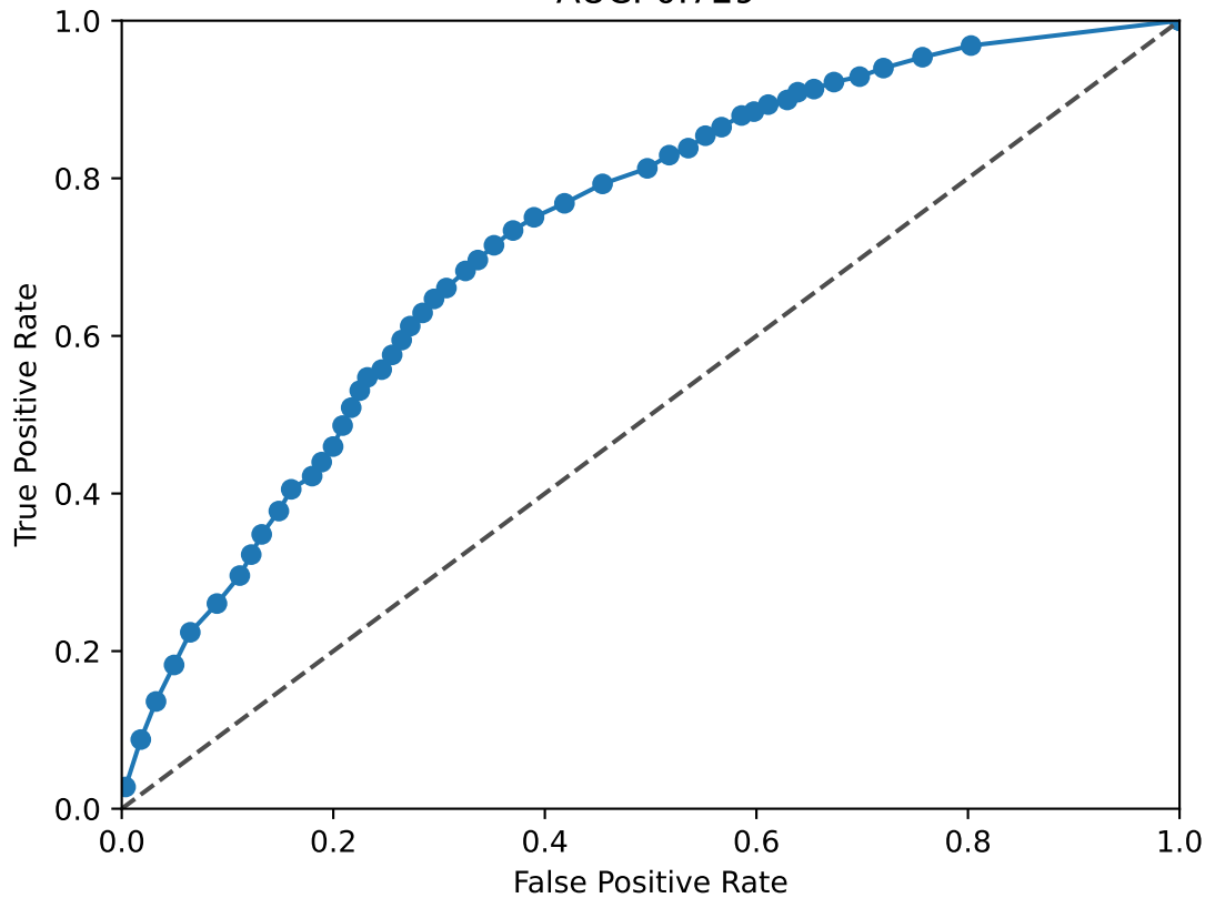
HSF2 ROC Curve AUC: 0.729
