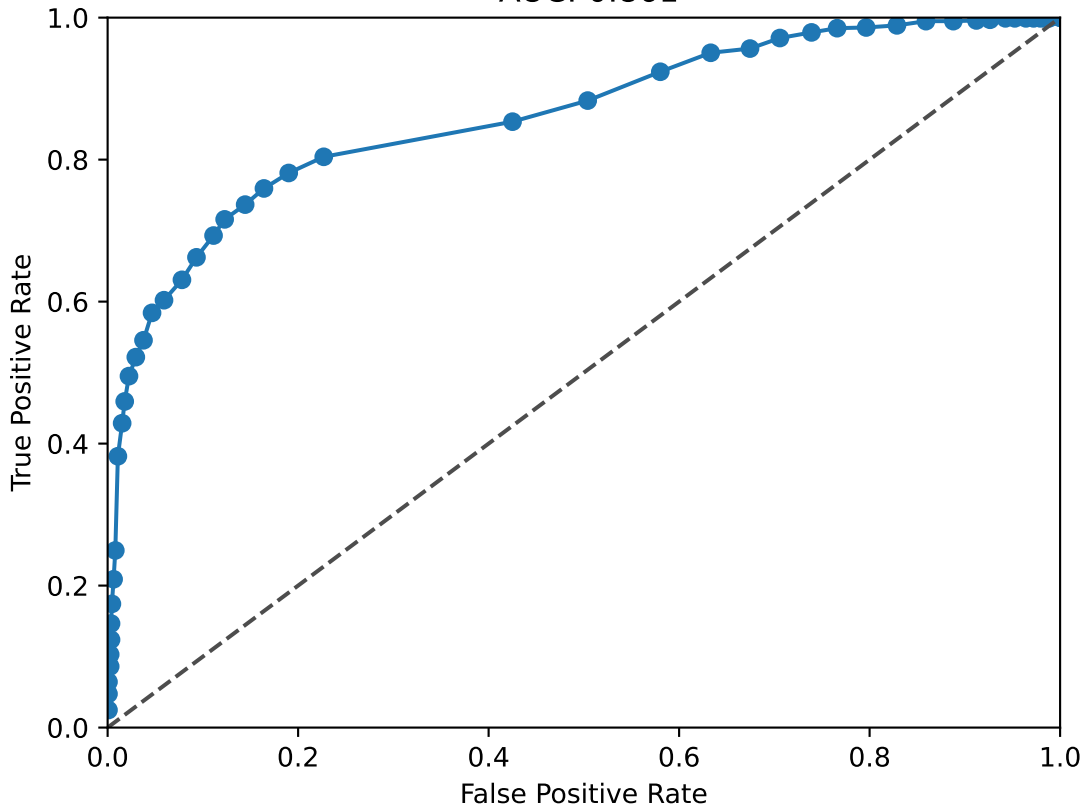
JUN ROC Curve AUC: 0.861
