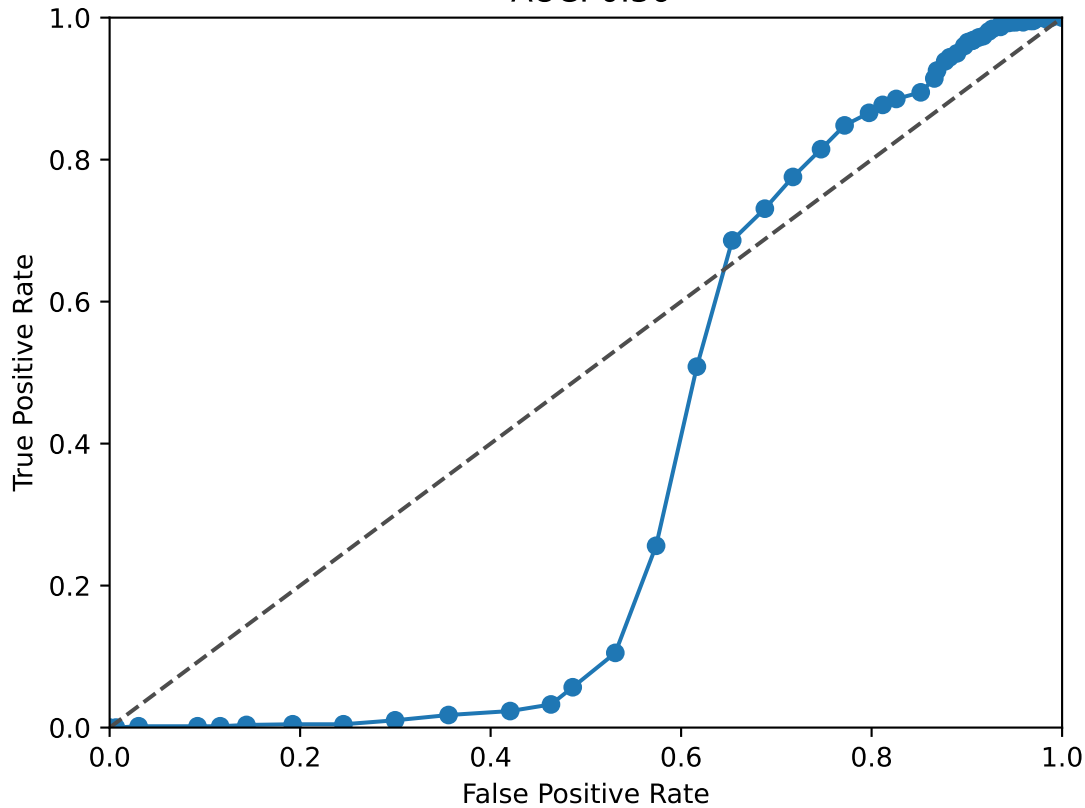
KMT2A ROC Curve AUC: 0.36
