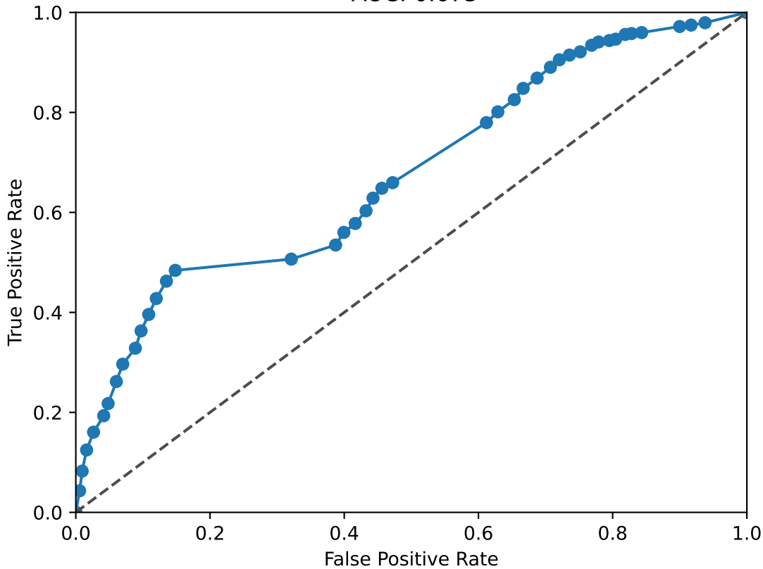
NFATC2 ROC Curve AUC: 0.675
