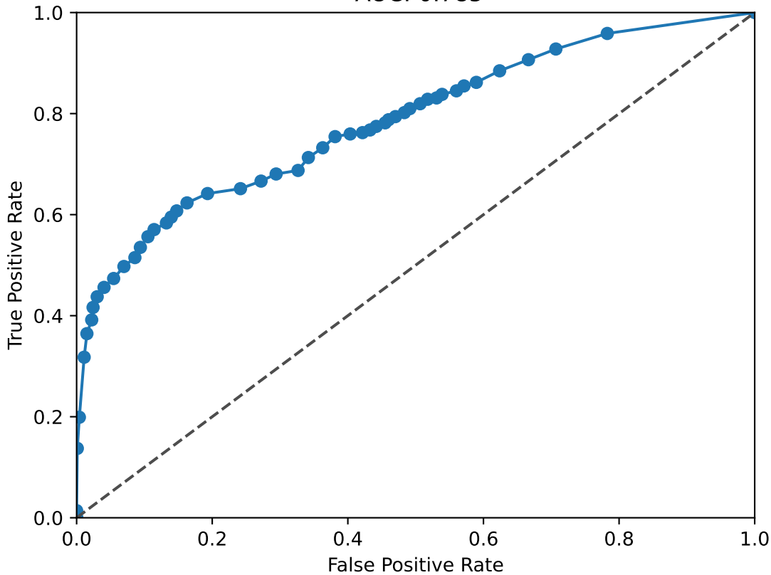
NFIA ROC Curve AUC: 0.785
