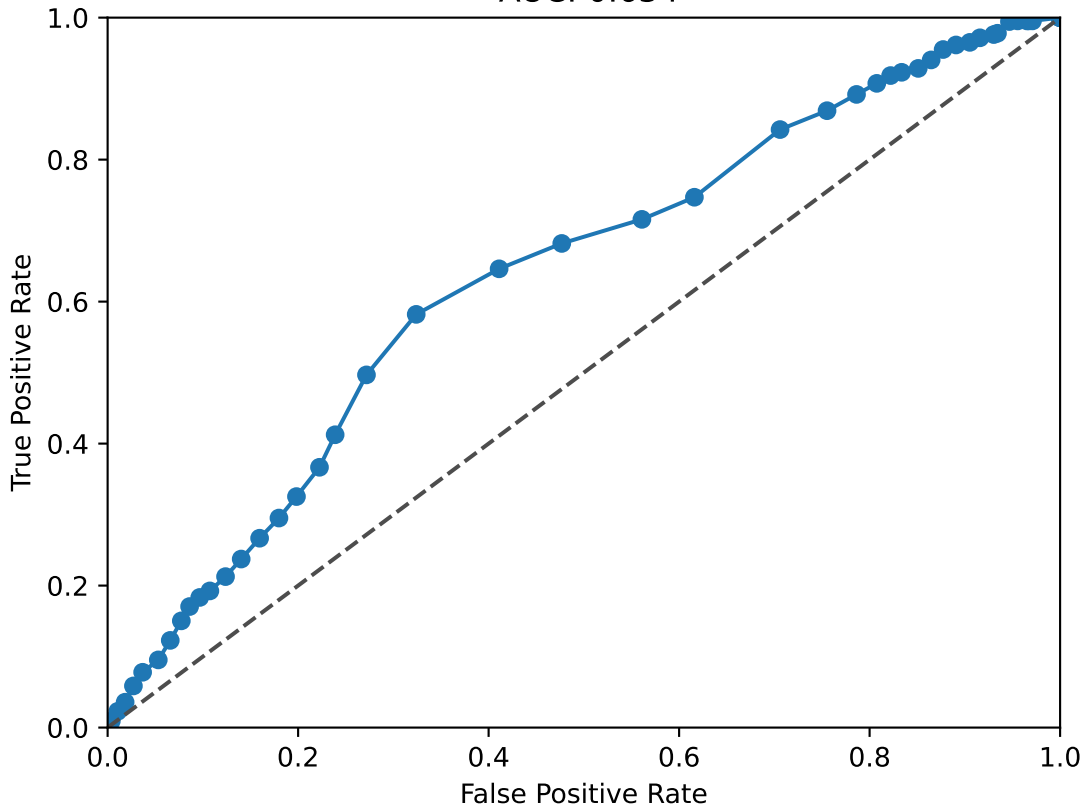
PBX1 ROC Curve AUC: 0.634
