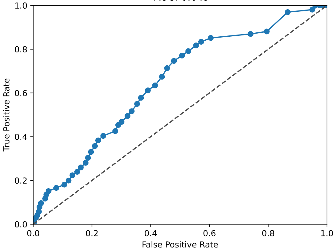
PKNOX2 ROC Curve AUC: 0.649
