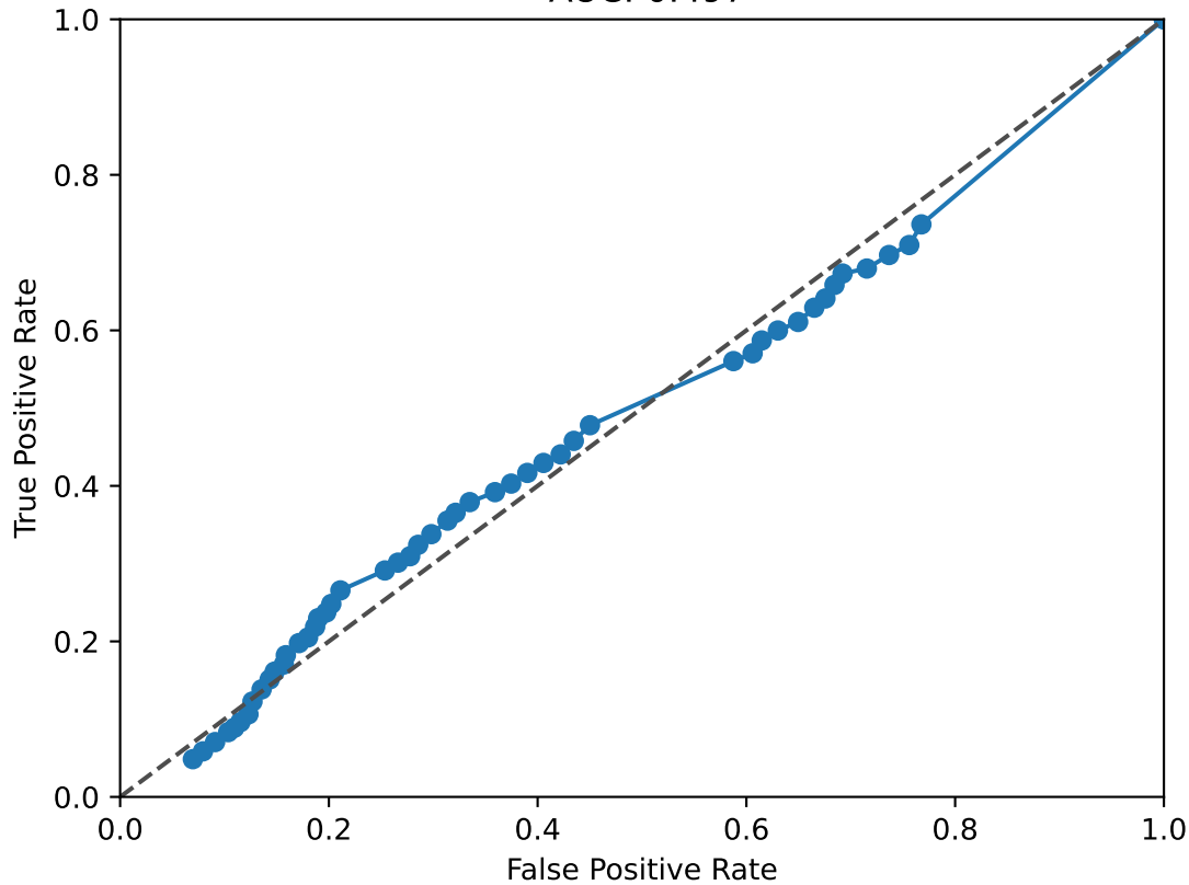
REST ROC Curve AUC: 0.497
